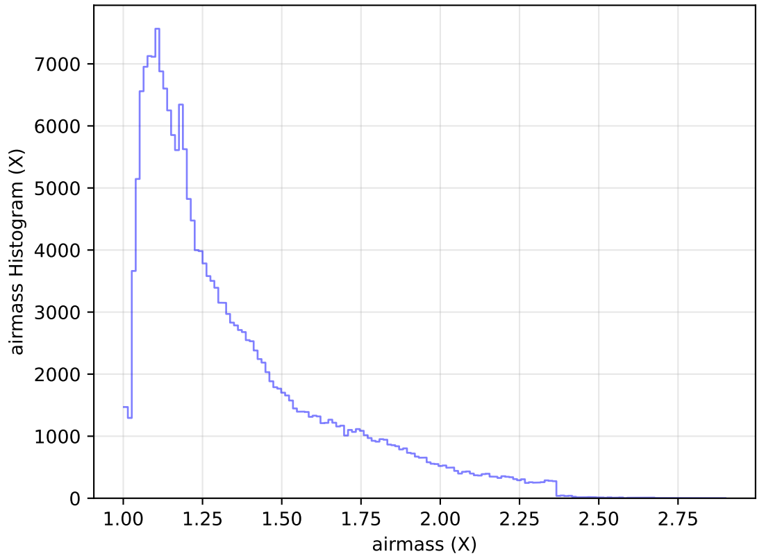
too_elab_heavy_r128_d2_griz_v3.4_10yrs All sky g band: airmass Histogram
