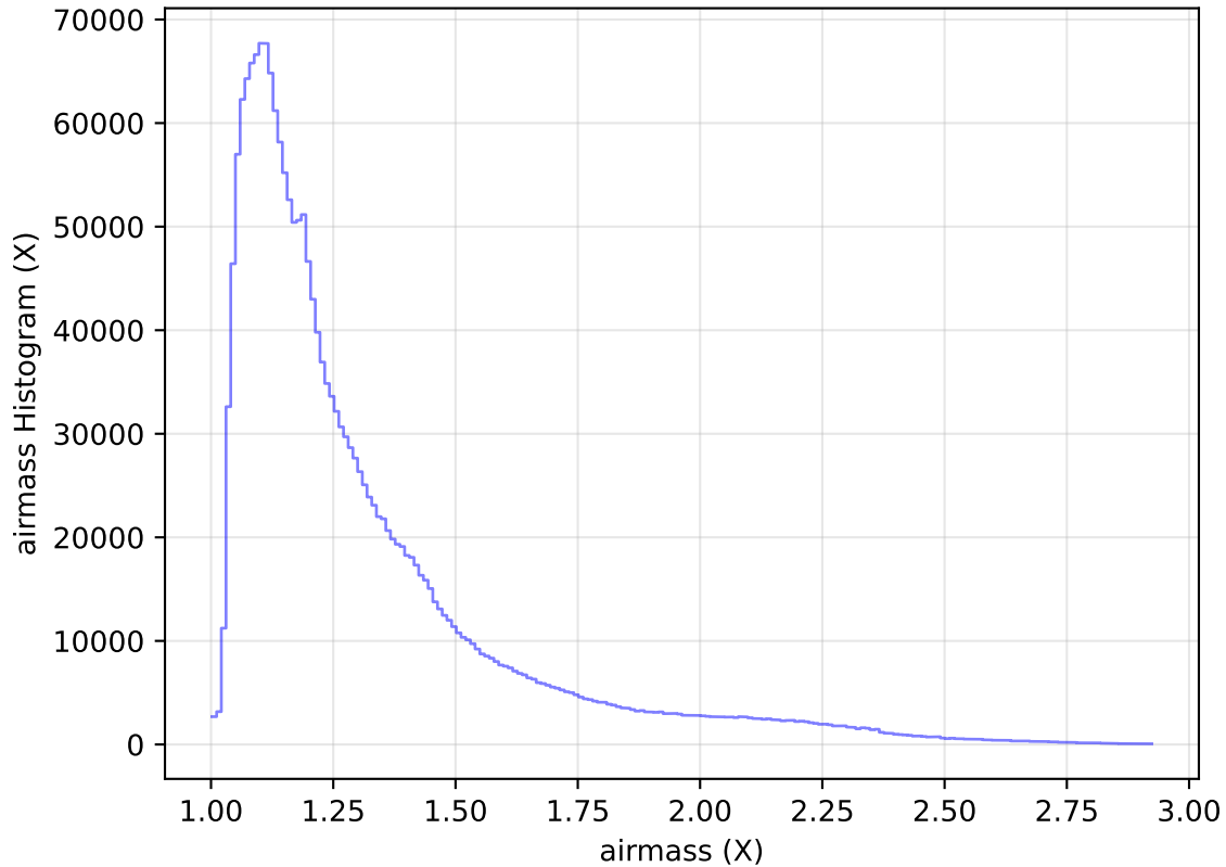
too_elab_heavy_r128_d2_griz_v3.4_10yrs All sky all bands: airmass Histogram
