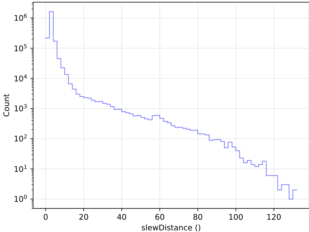
too_elab_heavy_r128_d2_griz_v3.4_10yrs All visits: Slew Distance Histogram
