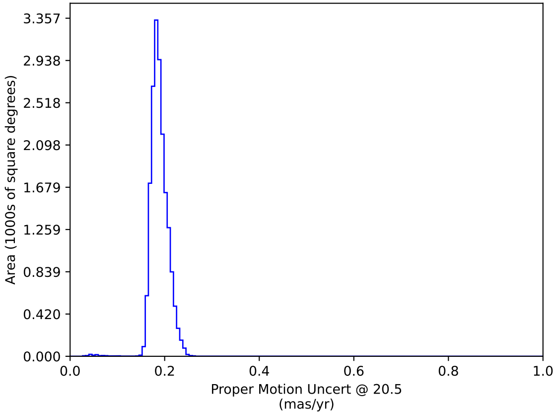
too_elab_heavy_r128_d2_griz_v3.4_10yrs WFD: Proper Motion Uncert @ 20.5
