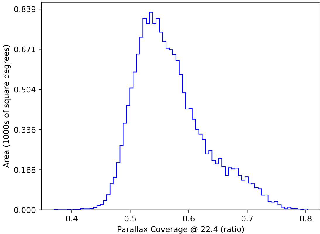
too_elab_heavy_r128_d2_griz_v3.4_10yrs WFD: Parallax Coverage @ 22.4
