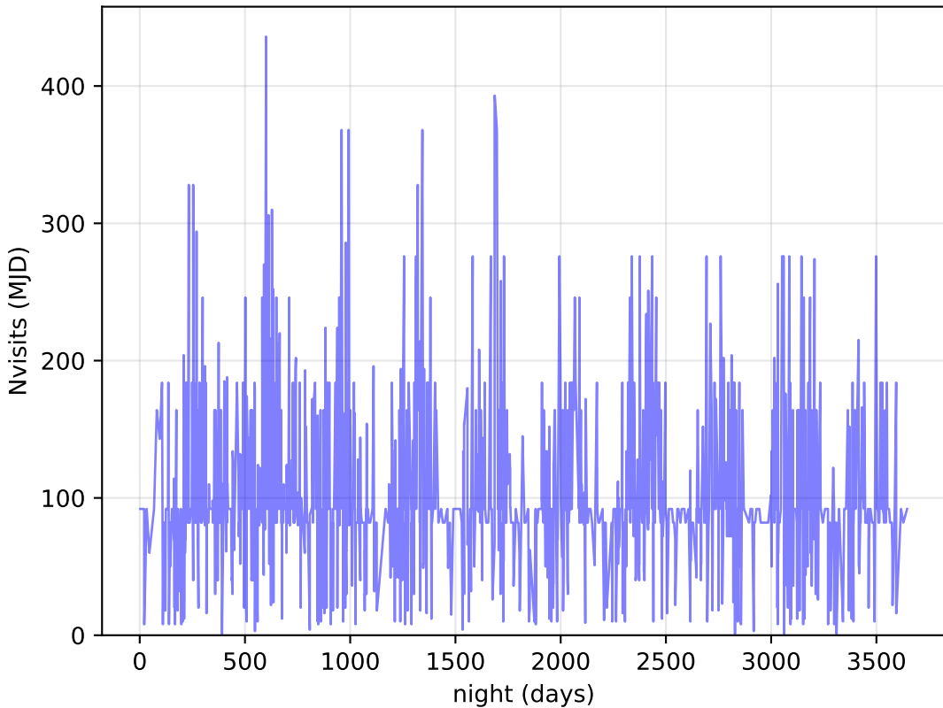
too_elab_heavy_r128_d2_griz_v3.4_10yrs DDF: Nvisits
