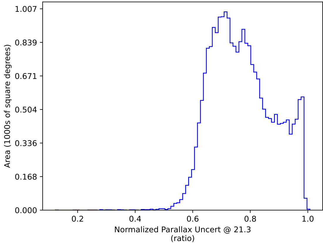
too_elab_heavy_r128_d2_griz_v3.4_10yrs All sky y band only: Normalized Parallax Uncert @ 21.3
