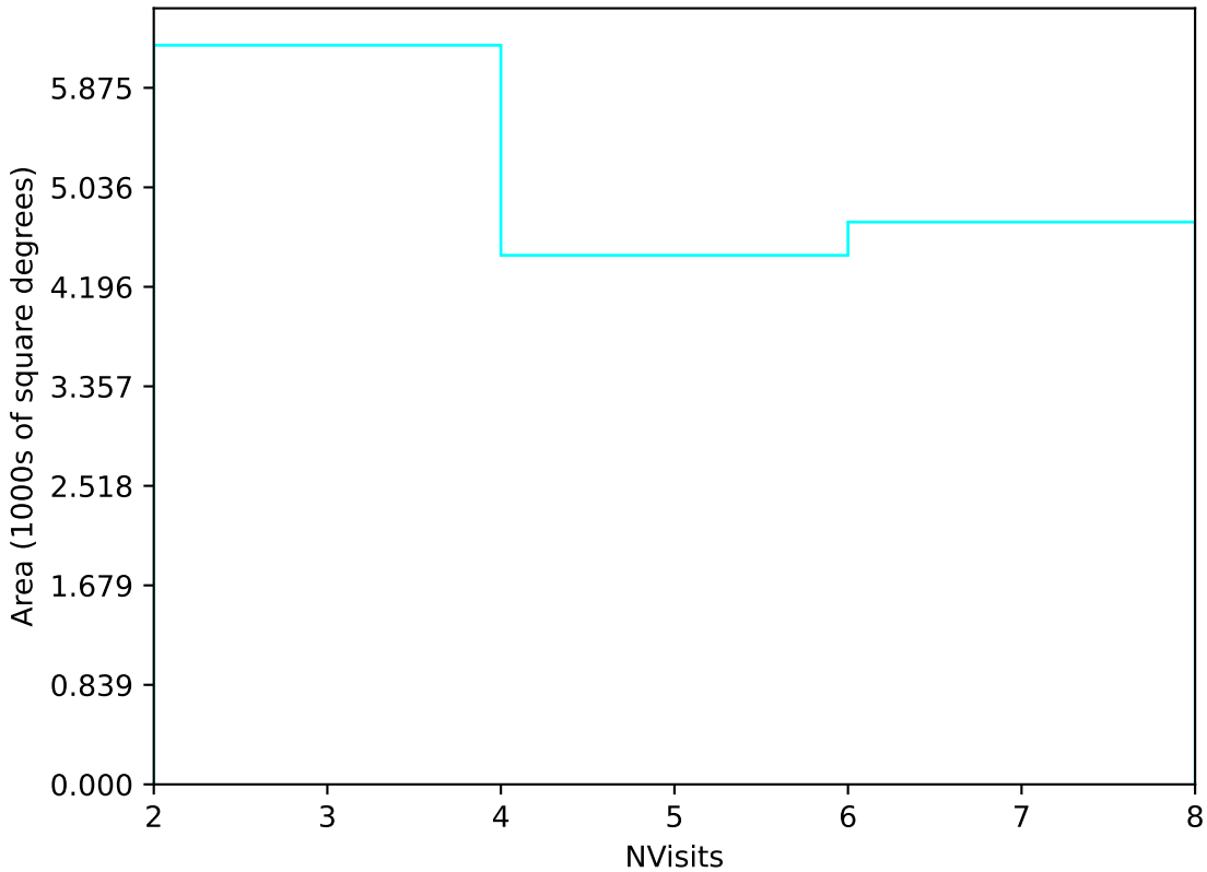
too_elab_heavy_r128_d2_griz_v3.4_10yrs Yr 3-4 u band: NVisits
