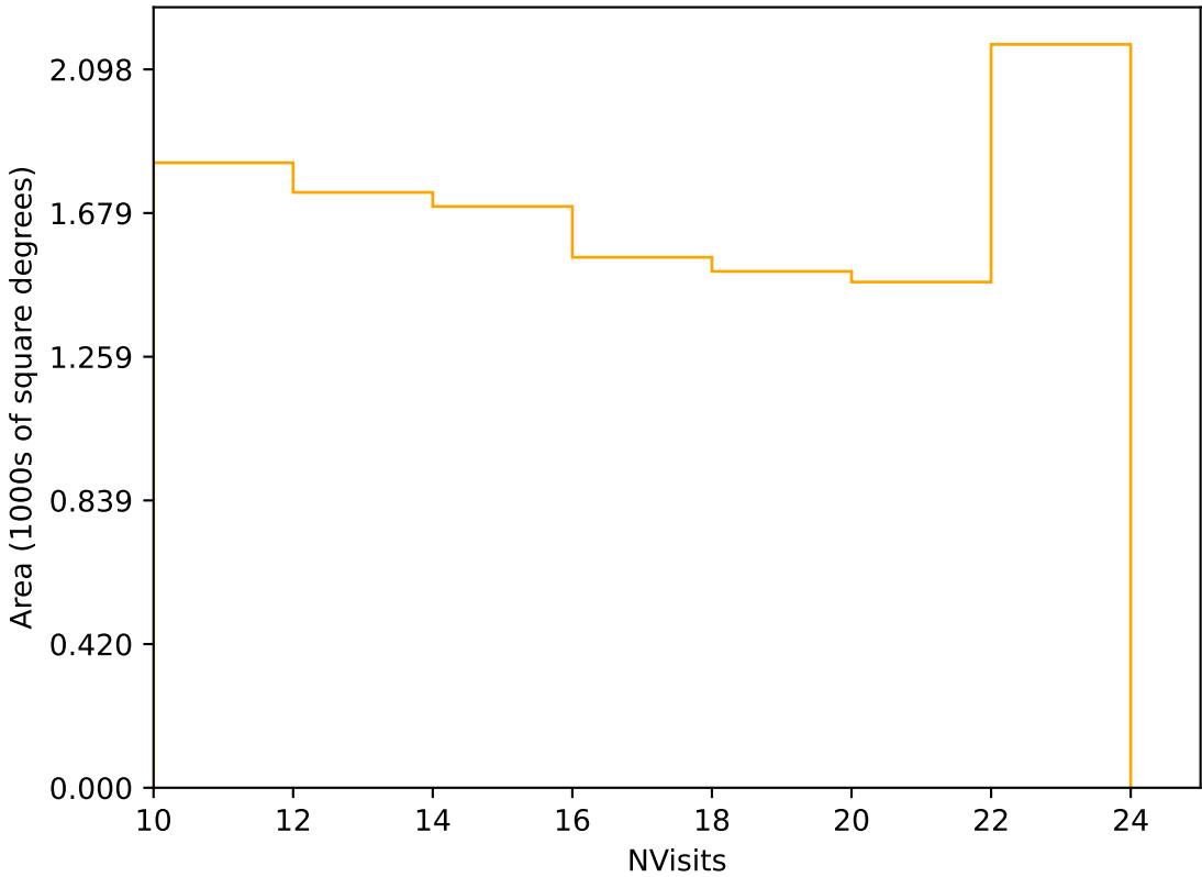
too_elab_heavy_r128_d2_griz_v3.4_10yrs Yr 3-4 r band: NVisits
