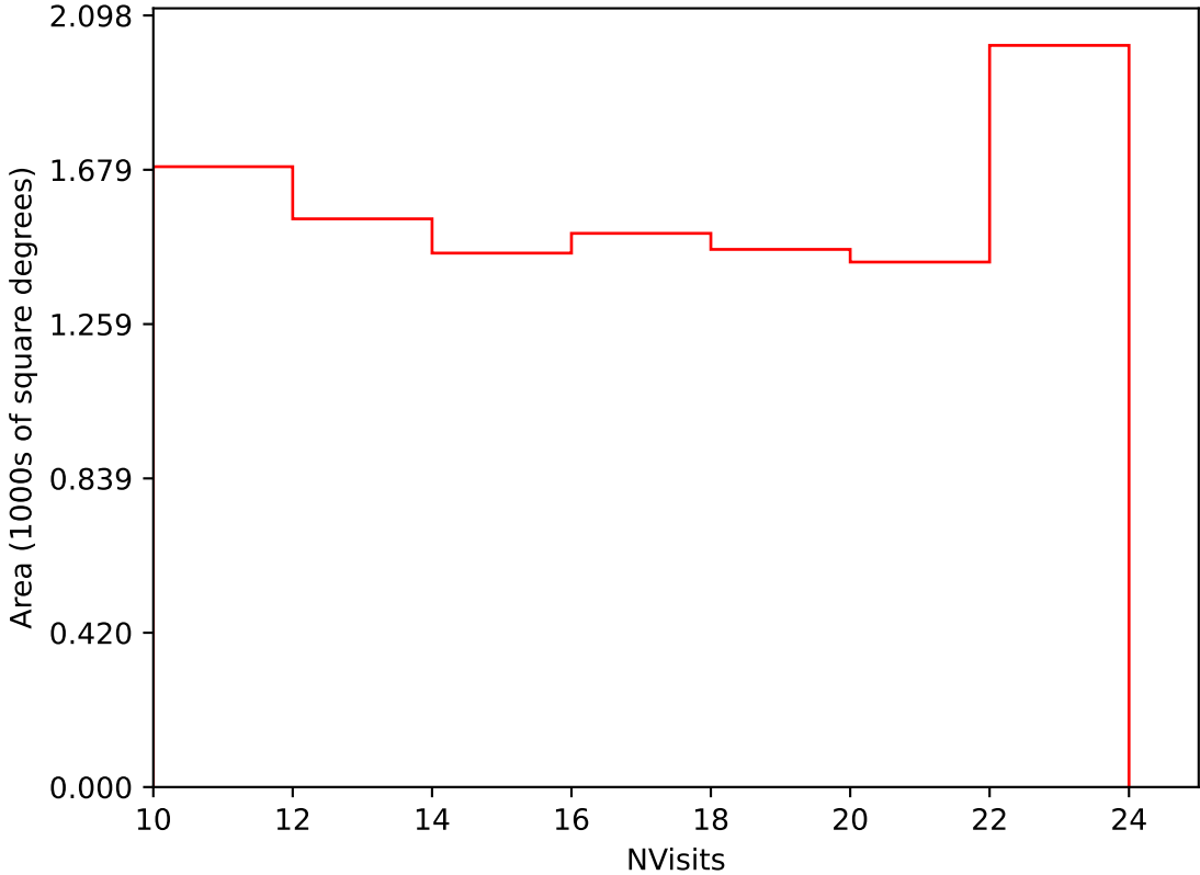
too_elab_heavy_r128_d2_griz_v3.4_10yrs Yr 3-4 i band: NVisits
