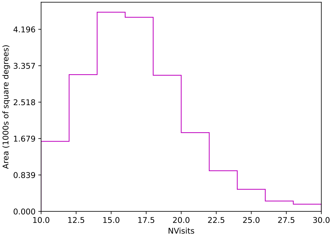
too_elab_heavy_r128_d2_griz_v3.4_10yrs Yr 1 z band: NVisits
