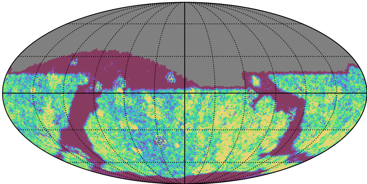
too_elab_heavy_r128_d2_griz_v3.4_10yrs Yr 1 i band: NVisits
