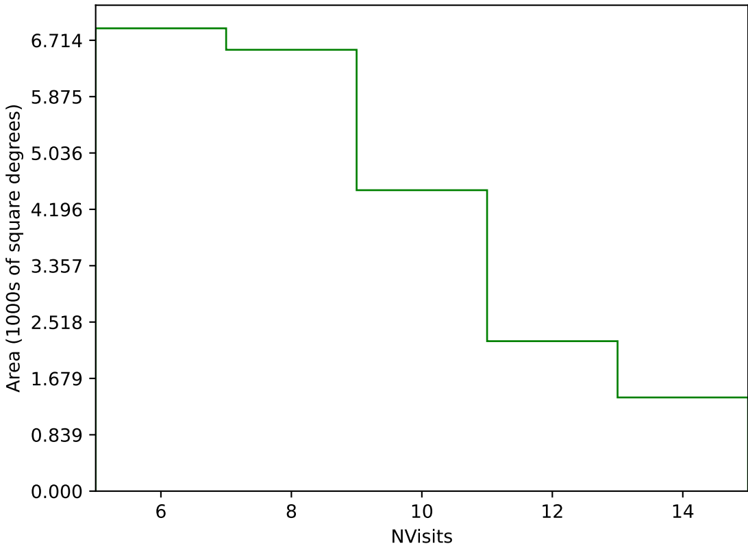
too_elab_heavy_r128_d2_griz_v3.4_10yrs Yr 1 g band: NVisits
