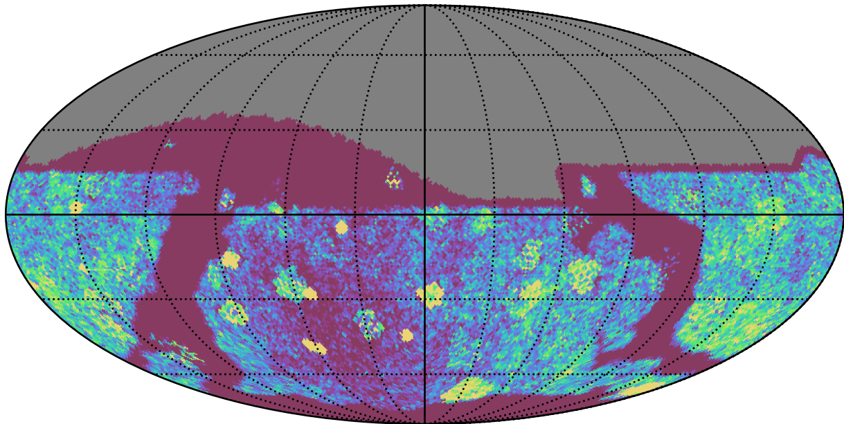
too_elab_heavy_r128_d2_griz_v3.4_10yrs Yr 1 all bands: NVisits
