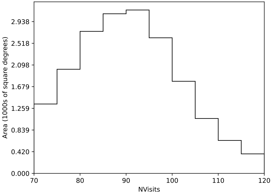
too_elab_heavy_r128_d2_griz_v3.4_10yrs Yr 1 all bands: NVisits
