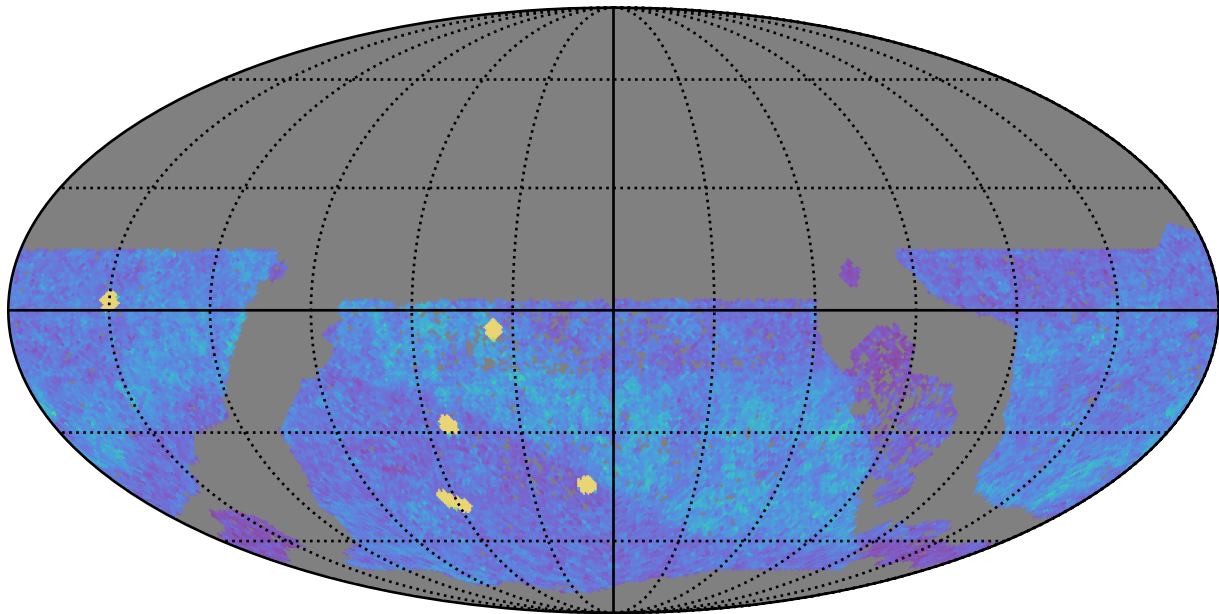
too_elab_heavy_r128_d2_griz_v3.4_10yrs WFD z band: NVisits
