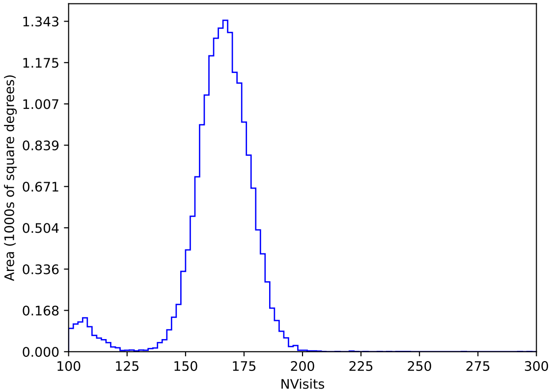
too_elab_heavy_r128_d2_griz_v3.4_10yrs WFD y band: NVisits
