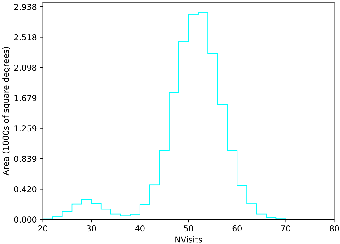
too_elab_heavy_r128_d2_griz_v3.4_10yrs WFD u band: NVisits
