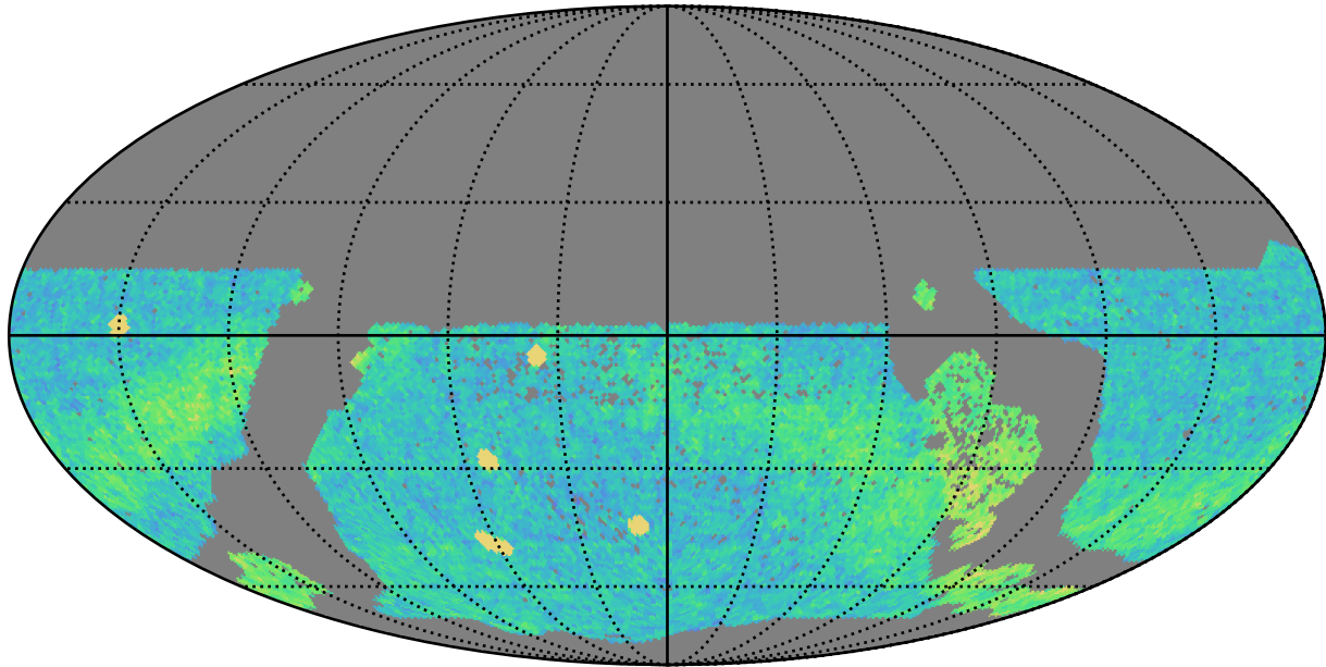
too_elab_heavy_r128_d2_griz_v3.4_10yrs WFD r band: NVisits
