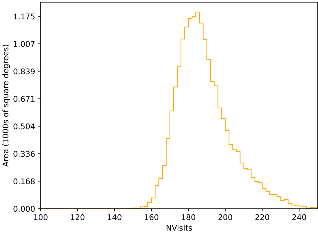
too_elab_heavy_r128_d2_griz_v3.4_10yrs WFD r band: NVisits
