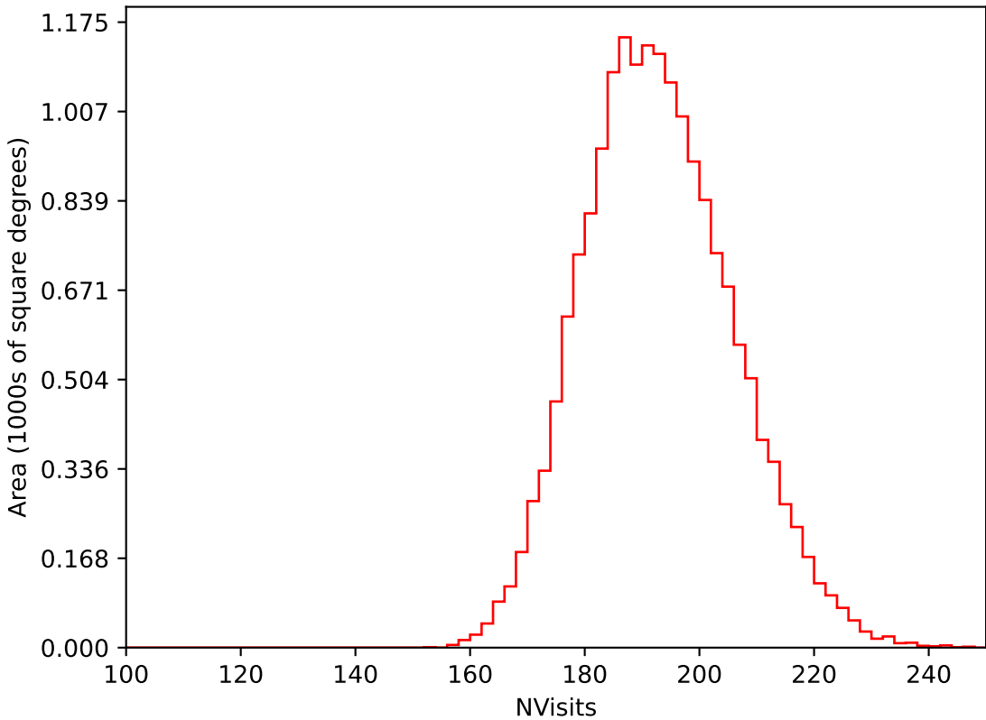
too_elab_heavy_r128_d2_griz_v3.4_10yrs WFD i band: NVisits
