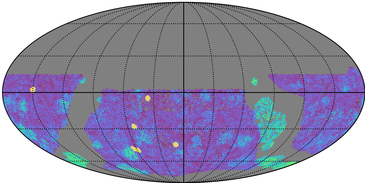
too_elab_heavy_r128_d2_griz_v3.4_10yrs WFD g band: NVisits
