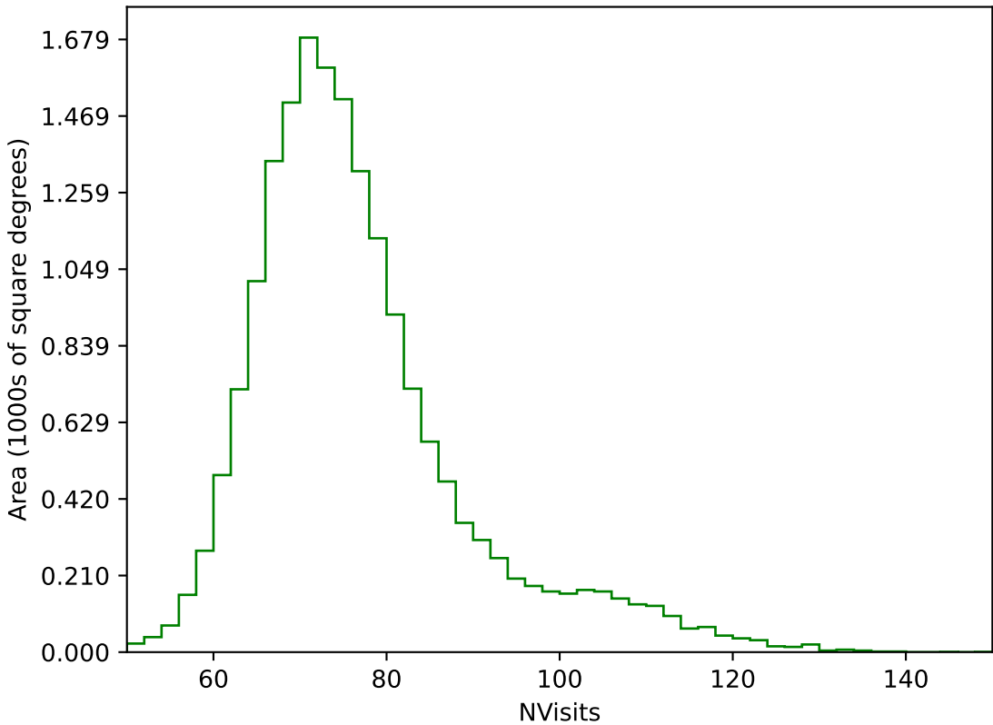
too_elab_heavy_r128_d2_griz_v3.4_10yrs WFD g band: NVisits
