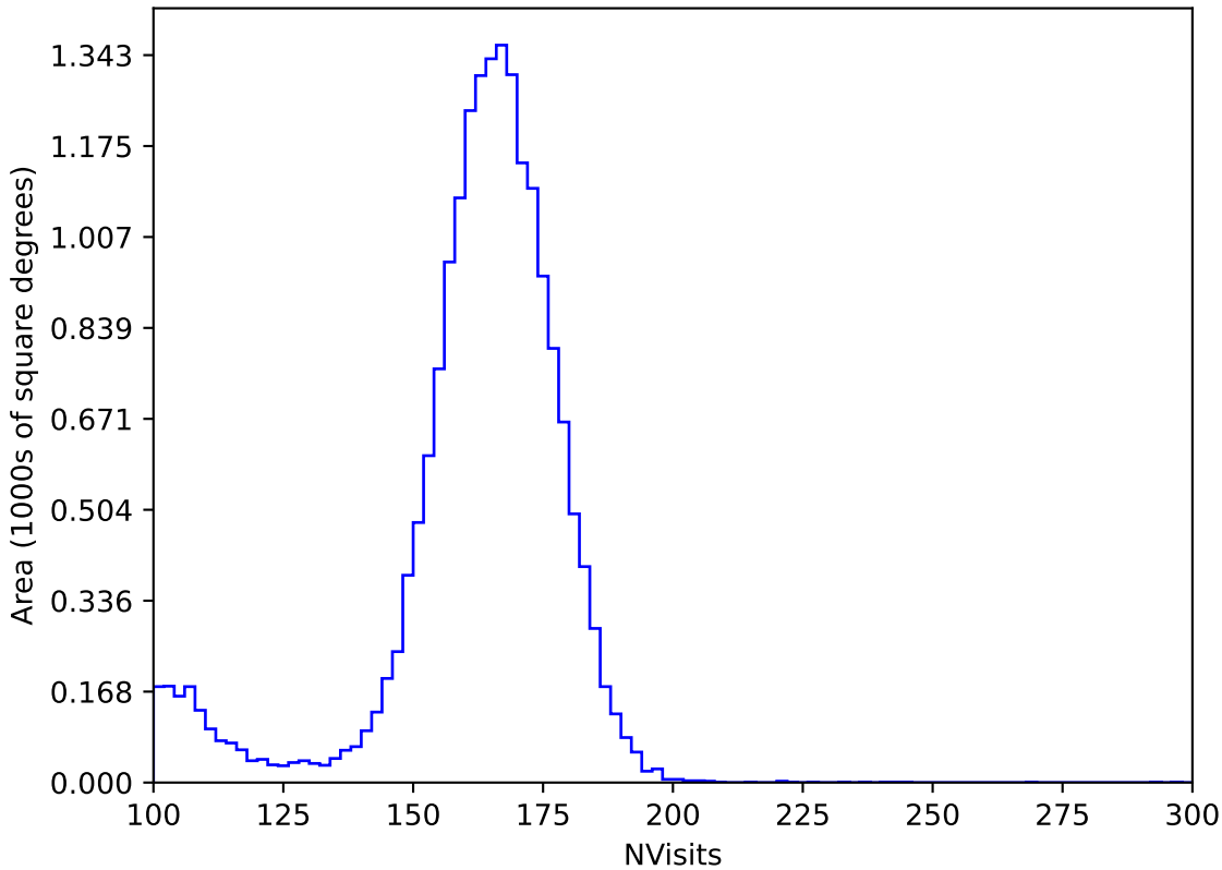
too_elab_heavy_r128_d2_griz_v3.4_10yrs All sky y band: NVisits
