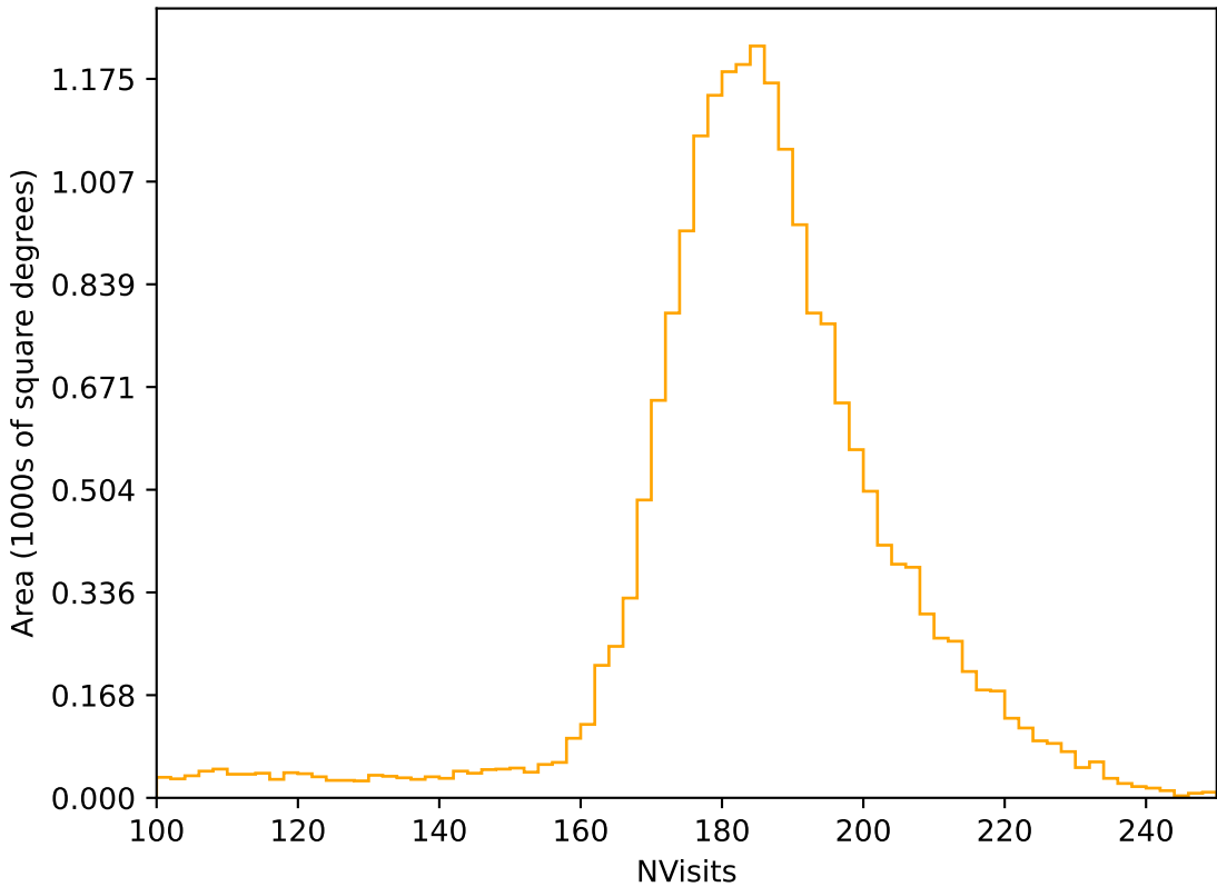
too_elab_heavy_r128_d2_griz_v3.4_10yrs All sky r band: NVisits
