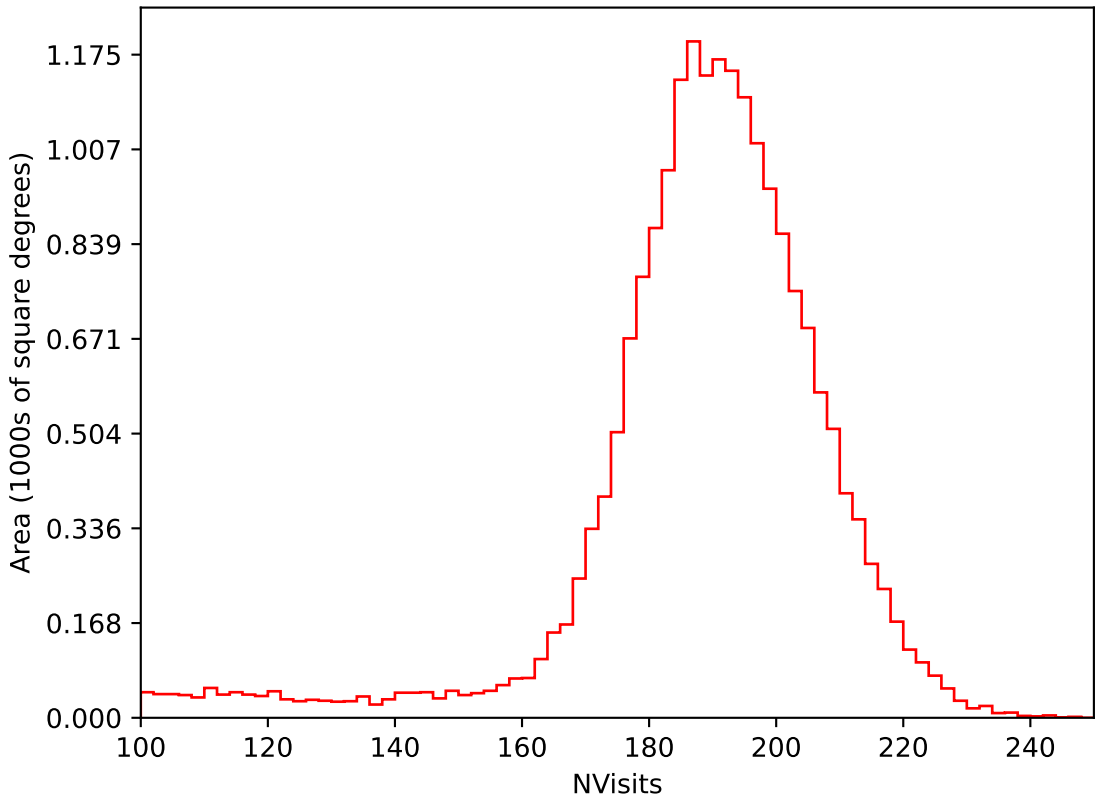
too_elab_heavy_r128_d2_griz_v3.4_10yrs All sky i band: NVisits
