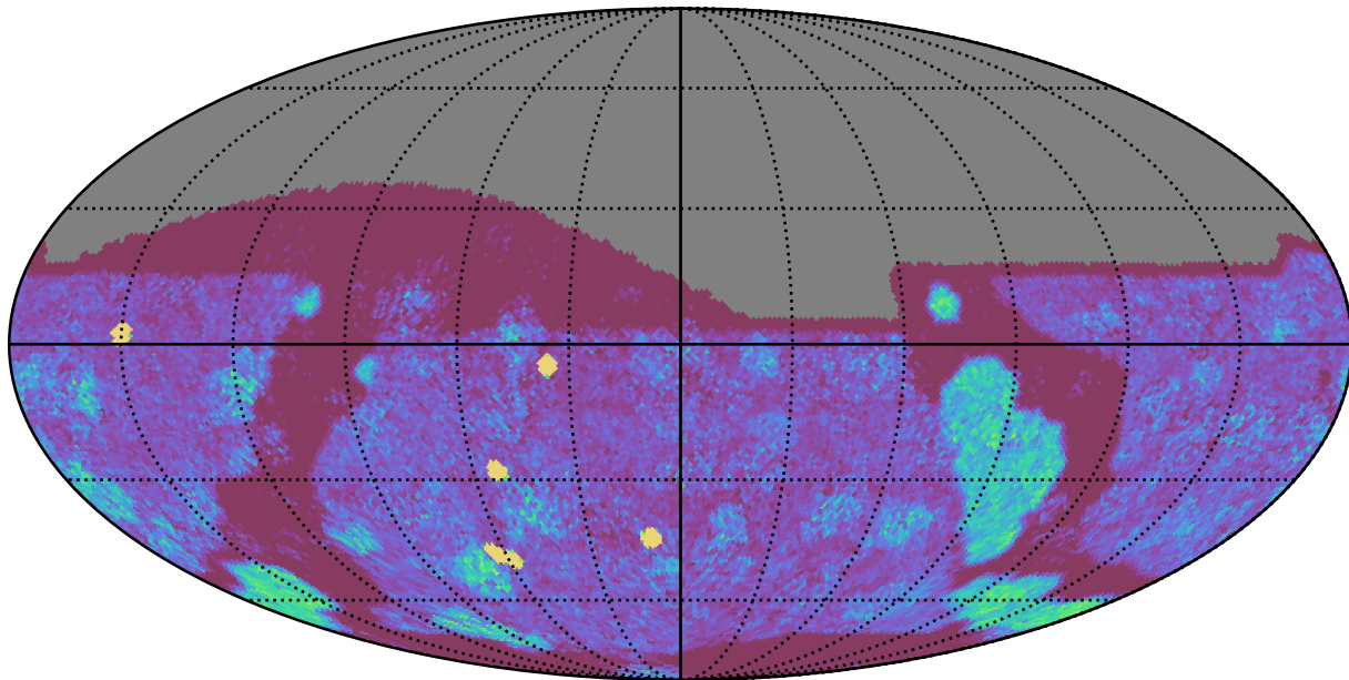
too_elab_heavy_r128_d2_griz_v3.4_10yrs All sky g band: NVisits
