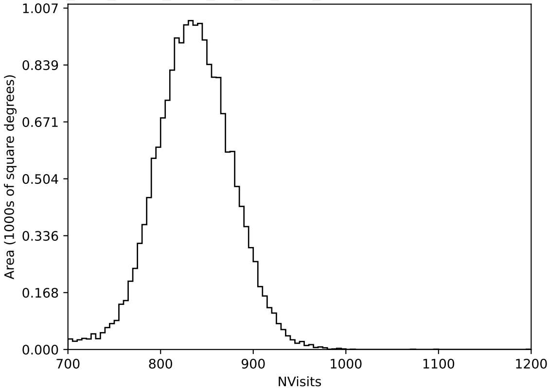
too_elab_heavy_r128_d2_griz_v3.4_10yrs All sky all bands: NVisits
