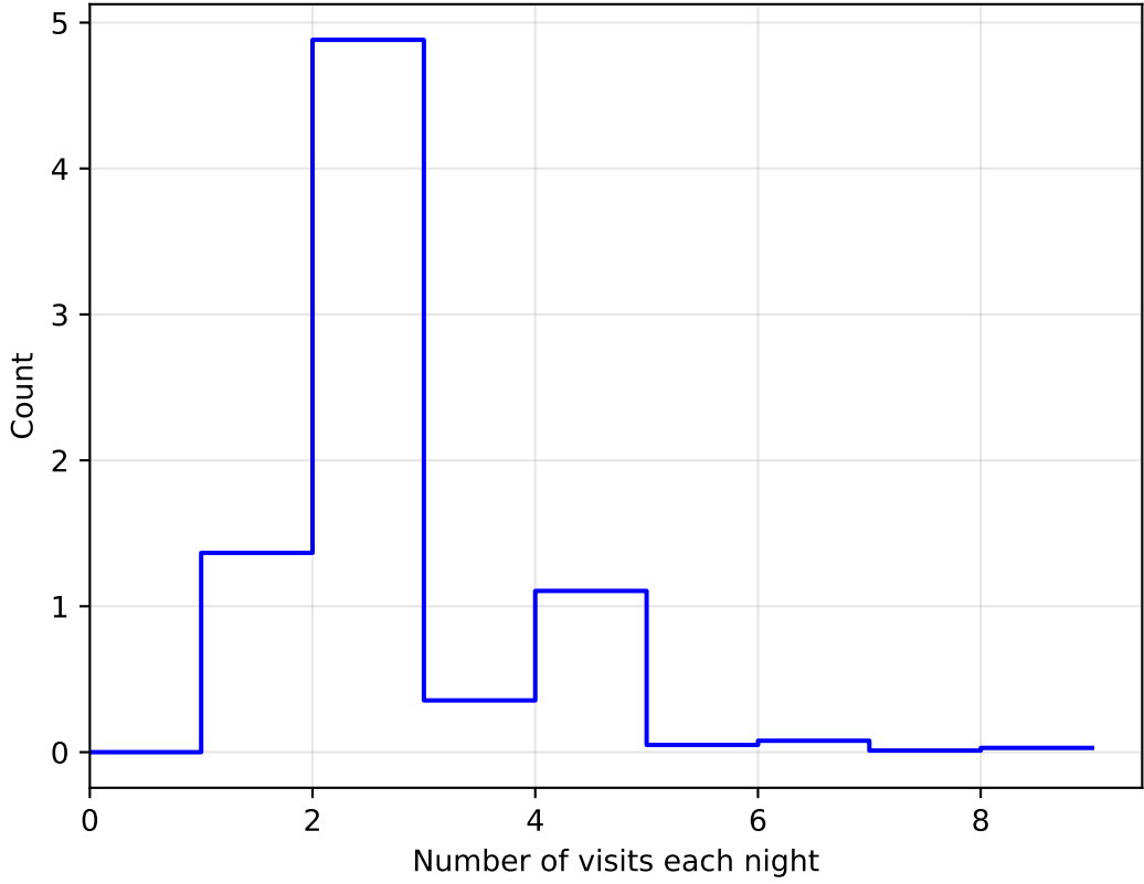
too_elab_heavy_r128_d2_griz_v3.4_10yrs WFD: NVisitsPerNight 1e6
