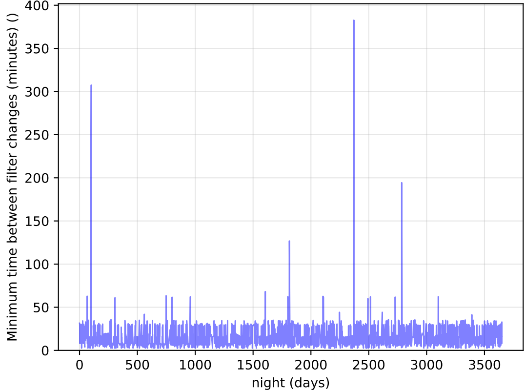
too_elab_heavy_r128_d2_griz_v3.4_10yrs Per Night: Minimum time between filter changes (minutes)
