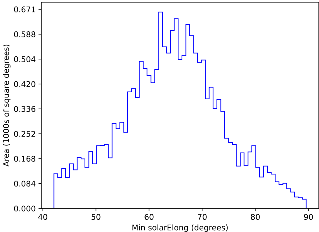
too_elab_heavy_r128_d2_griz_v3.4_10yrs WFD y band: Min solarElong
