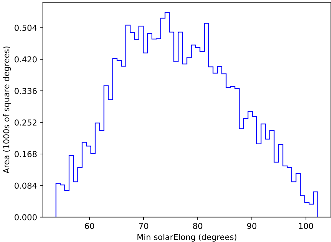
too_elab_heavy_r128_d2_griz_v3.4_10yrs WFD u band: Min solarElong
