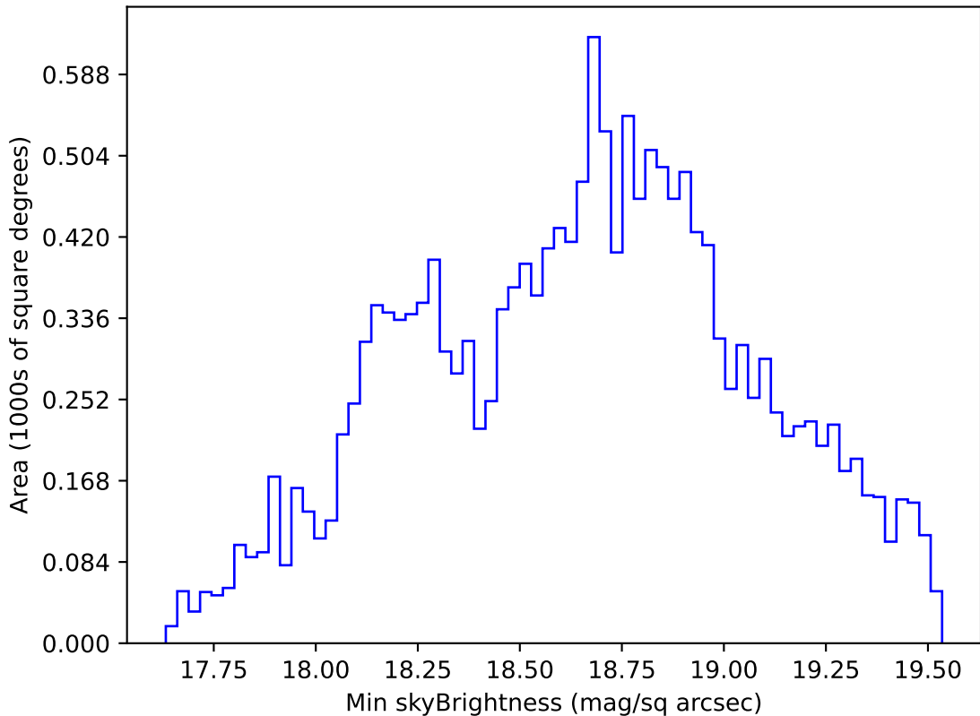
too_elab_heavy_r128_d2_griz_v3.4_10yrs WFD r band: Min skyBrightness
