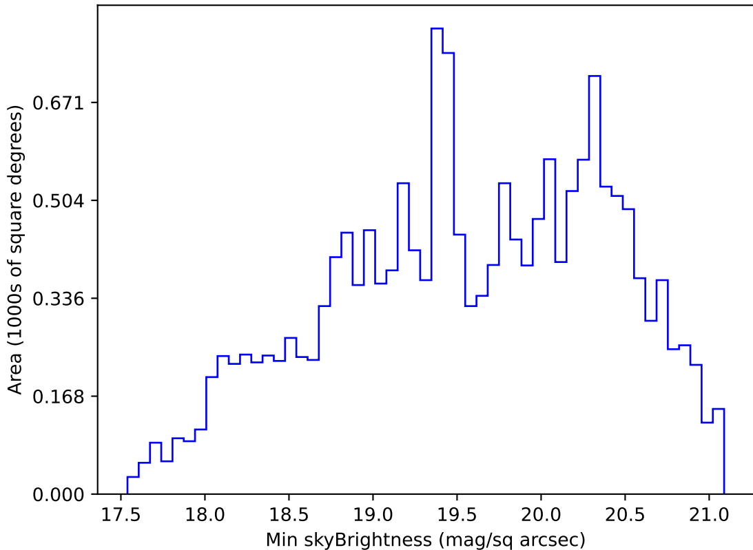
too_elab_heavy_r128_d2_griz_v3.4_10yrs WFD g band: Min skyBrightness
