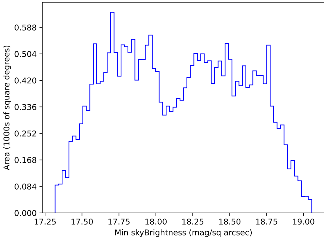
too_elab_heavy_r128_d2_griz_v3.4_10yrs All sky i band: Min skyBrightness
