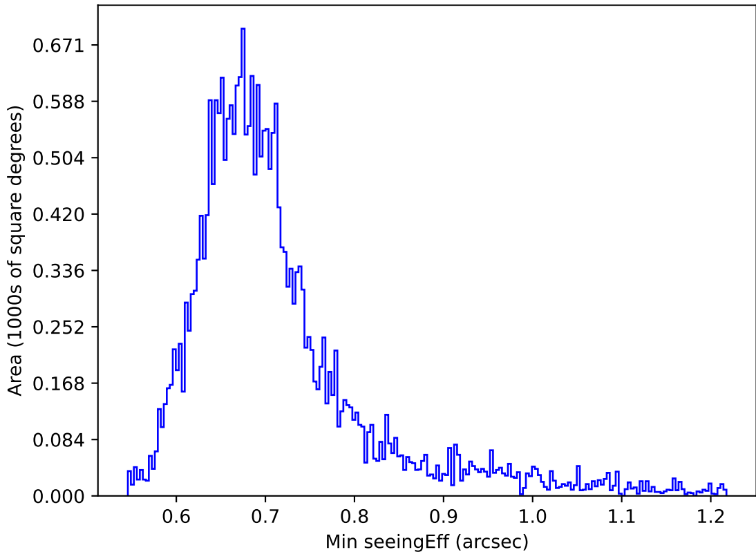
too_elab_heavy_r128_d2_griz_v3.4_10yrs Yr 1 i band: Min seeingEff
