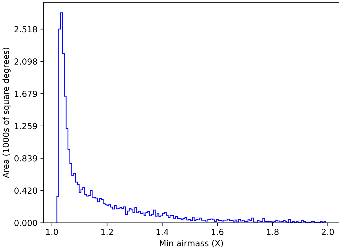
too_elab_heavy_r128_d2_griz_v3.4_10yrs Yr 1 i band: Min airmass
