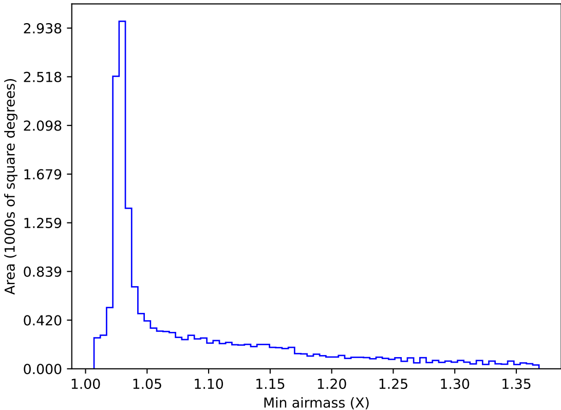
too_elab_heavy_r128_d2_griz_v3.4_10yrs WFD z band: Min airmass
