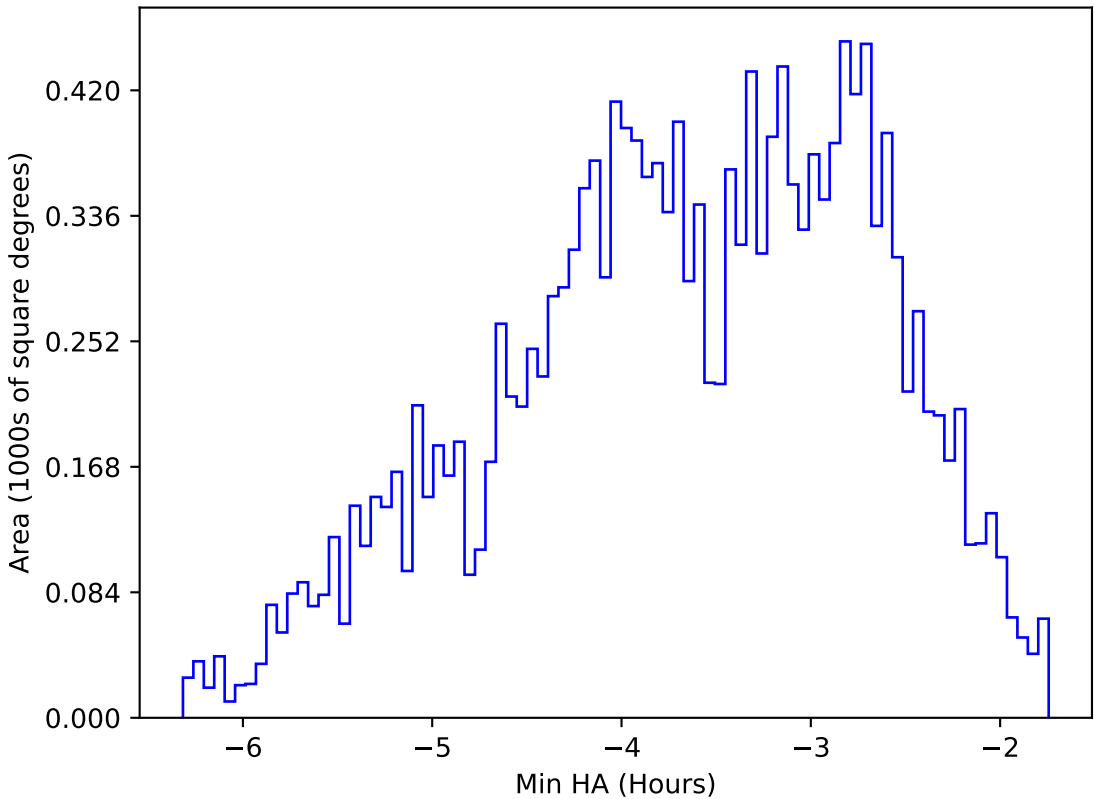
too_elab_heavy_r128_d2_griz_v3.4_10yrs WFD y band: Min HA
