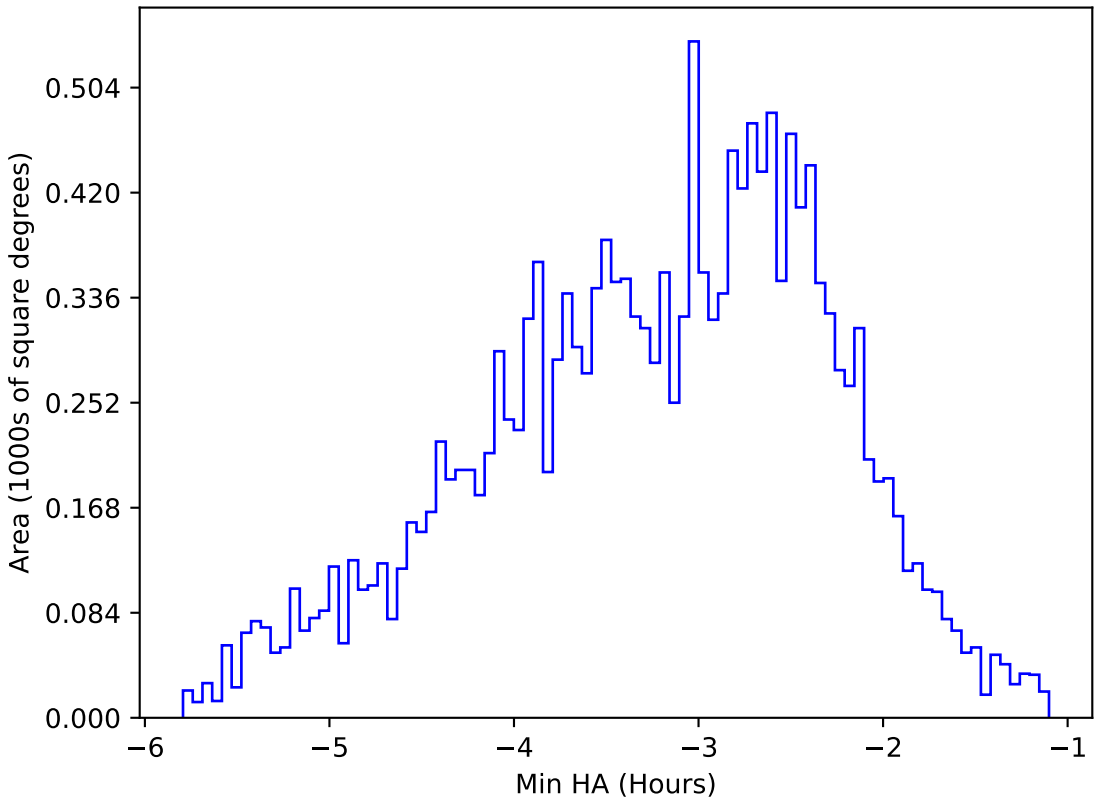
too_elab_heavy_r128_d2_griz_v3.4_10yrs WFD u band: Min HA
