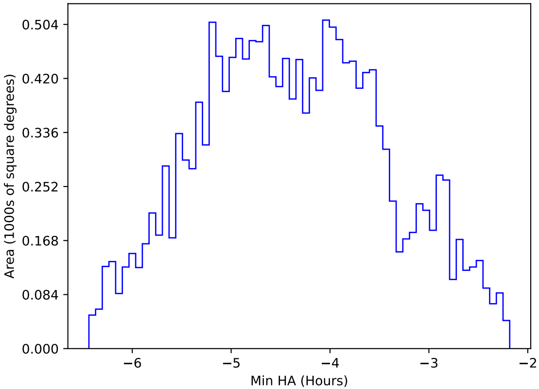
too_elab_heavy_r128_d2_griz_v3.4_10yrs WFD i band: Min HA
