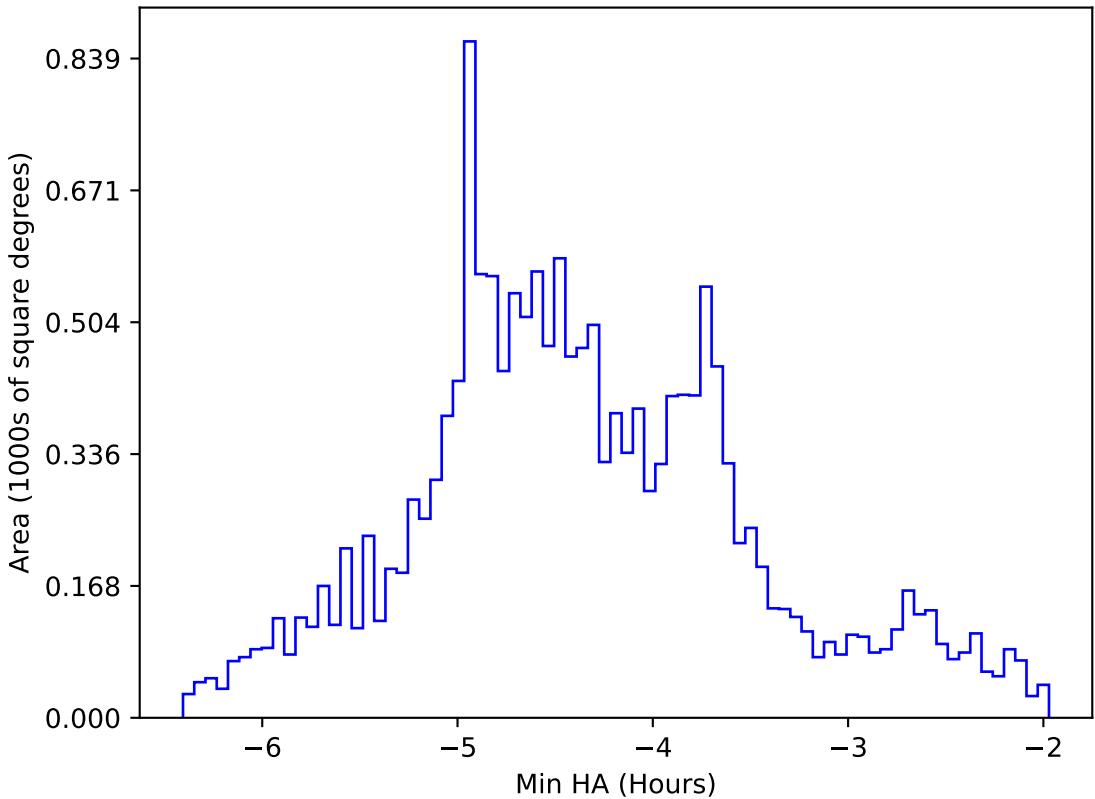
too_elab_heavy_r128_d2_griz_v3.4_10yrs WFD g band: Min HA
