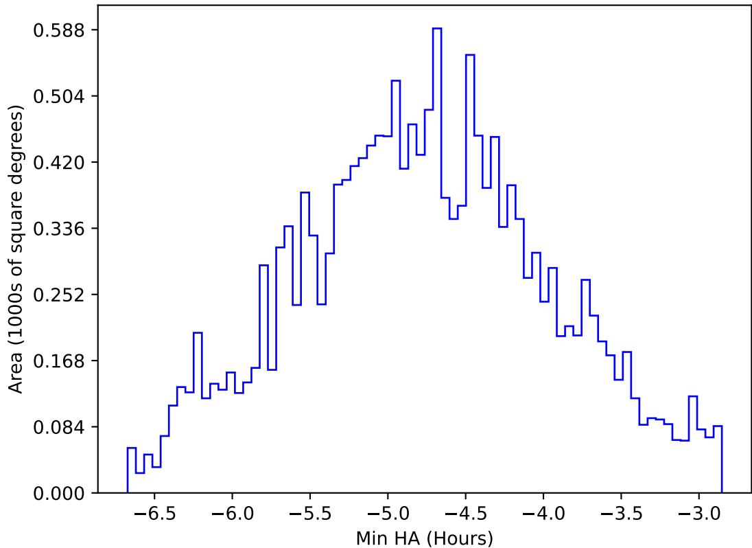
too_elab_heavy_r128_d2_griz_v3.4_10yrs WFD all bands: Min HA
