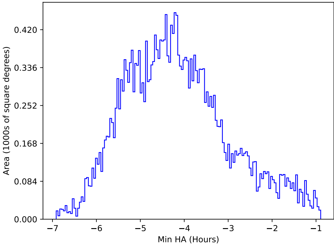
too_elab_heavy_r128_d2_griz_v3.4_10yrs All sky r band: Min HA
