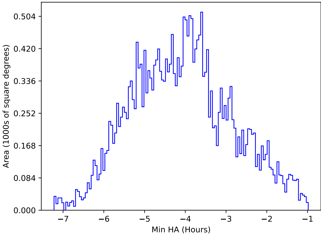
too_elab_heavy_r128_d2_griz_v3.4_10yrs All sky i band: Min HA
