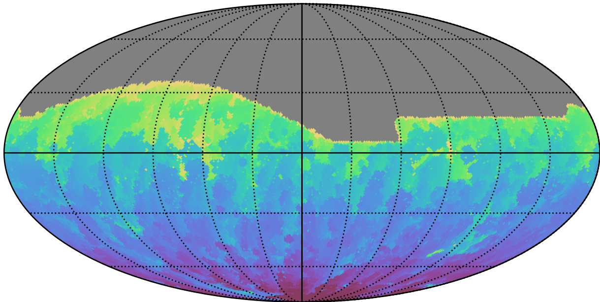
too_elab_heavy_r128_d2_griz_v3.4_10yrs All sky g band: Min HA
