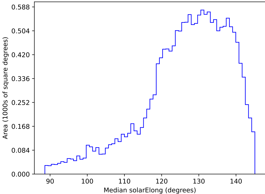
too_elab_heavy_r128_d2_griz_v3.4_10yrs WFD z band: Median solarElong
