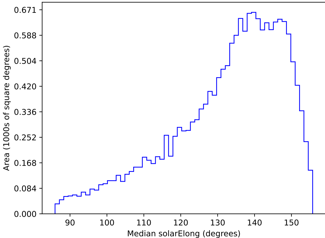
too_elab_heavy_r128_d2_griz_v3.4_10yrs WFD u band: Median solarElong
