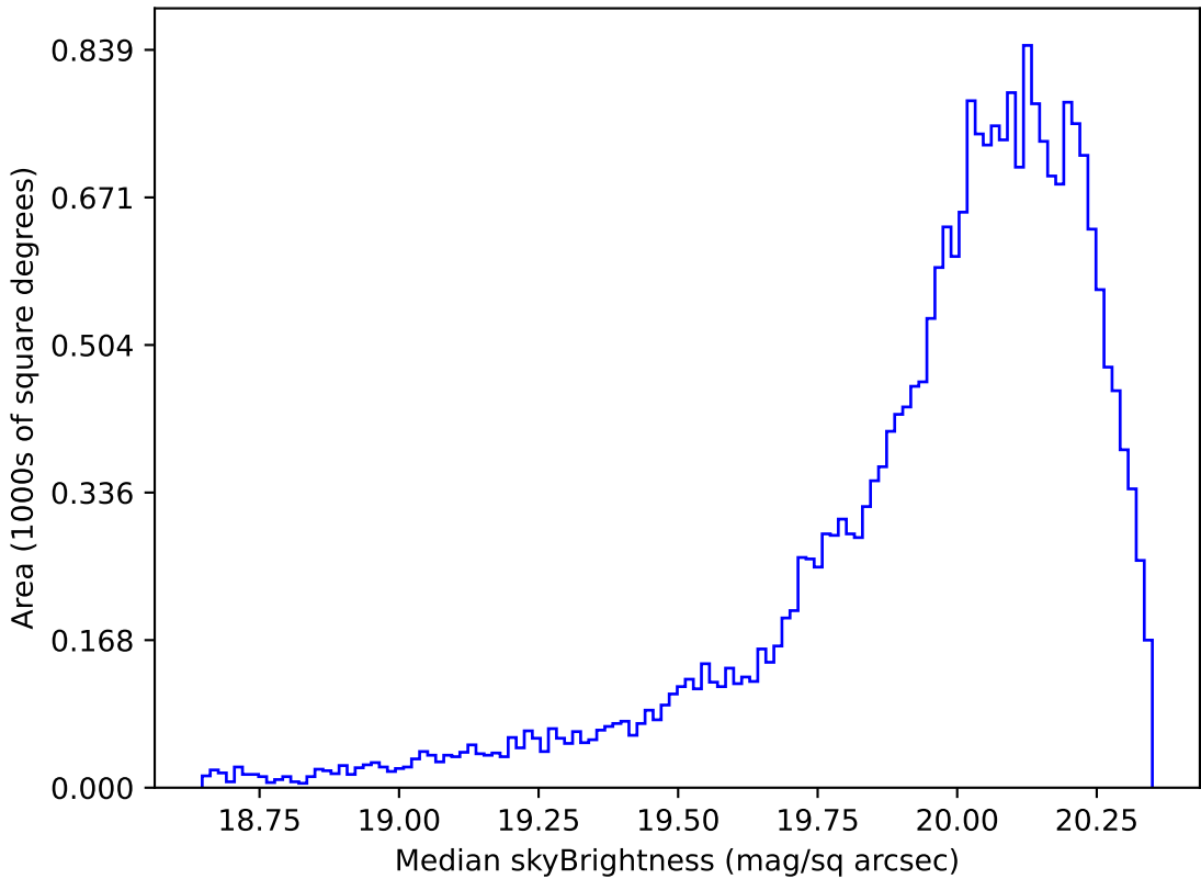
too_elab_heavy_r128_d2_griz_v3.4_10yrs Yr 1 i band: Median skyBrightness
