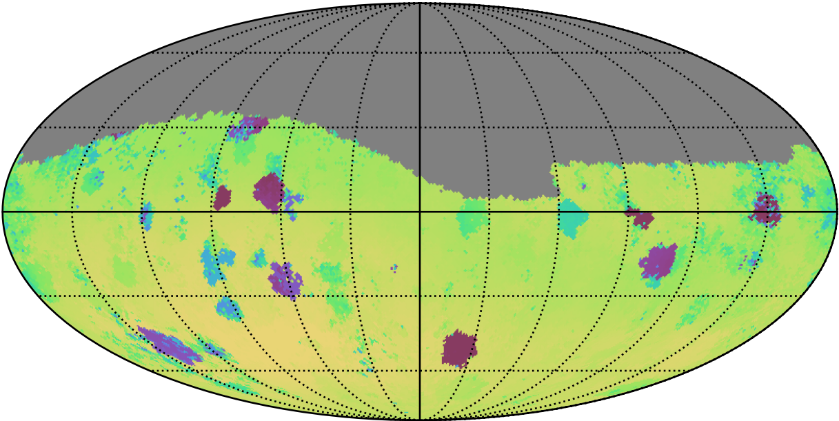
too_elab_heavy_r128_d2_griz_v3.4_10yrs Yr 1 g band: Median skyBrightness
